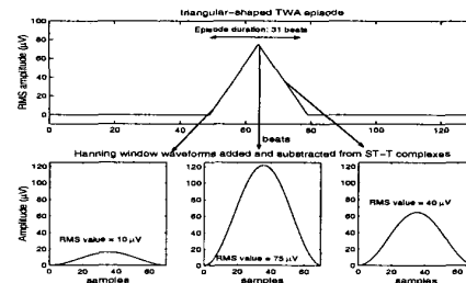
Figure 1. Simulated TWA episodes and waveforms.
