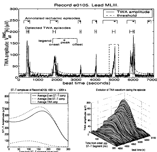
Figure 3. Top: Example of V_{rms}^{alt}[k] series for record e0105, showing annotated ischemic episodes, detected TWA, and adaptive threshold. Bottom: mean ST-T complexes and TWA (left) and TWA waveform evolution (right) of the episode marked with a the dotted box in the top panel.
