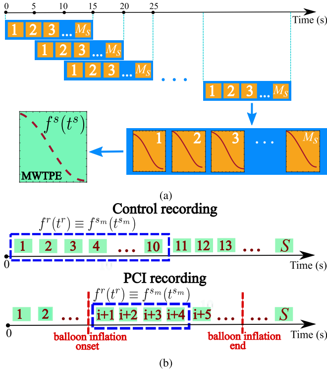
Fig. 1. MWTPE f^s(t^s) estimation and reference MWTPE f^r(t^r) selection rule at the STAFF-III data-set. The f^s(t^s) MWTPE was estimated from time-windows of 15 seconds duration and 10 seconds of overlap throughout the entire record. The reference f^r(t^r) MWTPE was selected among the MWTPEs within 1 minute period, at the control recording, and within 30 seconds period at the beginning of the PCI recordings.
