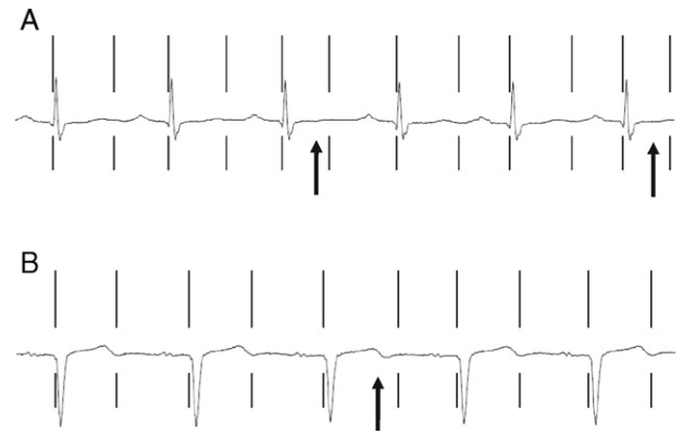
Fig. 2. Examples of leads discarded because of unstable delineation. A, EASI-derived lead II. The QT intervals of the third and last beats are considerably shorter than of the remaining beats, caused by very low T-wave amplitudes. B, Standard lead V 2 . All T waves were considered to be positive except the third one whose morphology was biphasic, thus, causing unstable QT-interval measurements.
