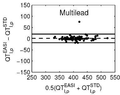
Fig. 4. Bland-Altman plot for the QT multilead measurements in EASI-derived and standard leads ( QT_{I,p}^{EASI} and QT_{I,p}^{STD} ). Dashed line indicates mean difference; solid lines, mean \pm 2 SDs.
