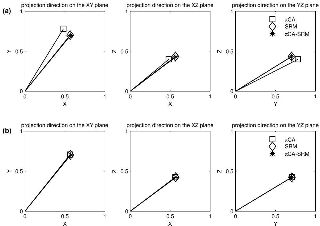
Fig. 4. Average direction of the projections obtained with the \pi CA scheme (squares), the SRM scheme (diamonds) and the \pi CA-SRM scheme (asterisks) in signals with (a) V_{alt}=10 \mu\text{V} and (b) V_{alt}=60 \mu\text{V} .
