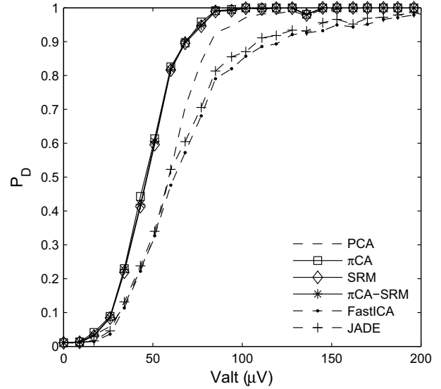
Fig. 3. P_D of the different schemes vs. simulated TWA amplitude. P_{FA} = 0.01 for all schemes.
