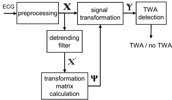
Fig. 2. Block diagram of the multilead scheme.
