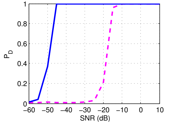
Figure 5: P_D for P_{FA} = 0.01 of the multilead (solid line) and the single-lead scheme (dashed line) vs. SNR.
