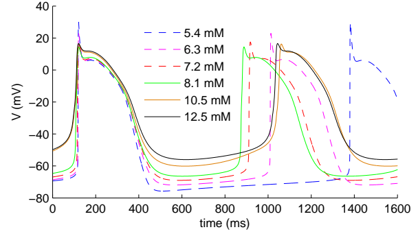
Figure 3. Spontaneous APs vs. [K^+]_o in isolated PK cells. Traces were extracted from the last two seconds of each simulation and aligned for illustration purposes.
