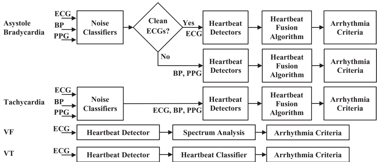
Fig. 1: Algorithm Overview
