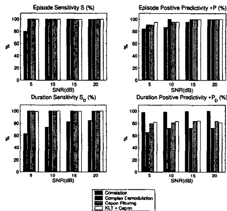
Fig. 4. Detection rate parameters for 'em' noise and 150 \mu\text{V} TWA amplitude.
