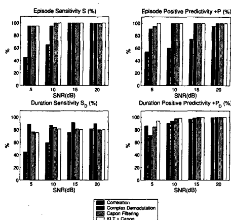
Fig. 7. Detection rate parameters for 'em' noise and 25 \mu V TWA amplitude.
