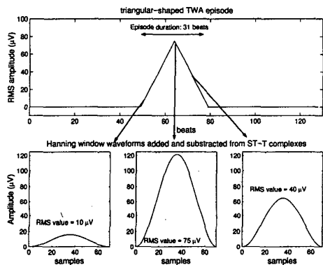
Fig. 3. Simulated TWA alternans episodes and waveforms.
