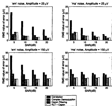
Fig. 8. Amplitude accuracy of the detectors.
