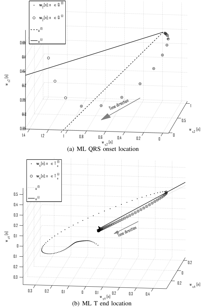
Fig. 3. Example of ML delineation (files from CSEDB database [9]): WT loops and the direction of the best line fit at the initial and final step (i = 2).
