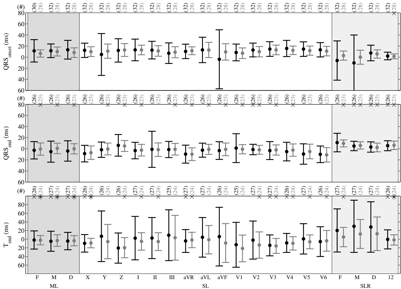
Fig. 5. Delineation results in CSEDB: comparison between ML over lead subsets F , M and D (darker grey area), SL over each of the 15 available leads and SLR over the standard 12 leads and over the 3 orthogonal leads in F , M and D (lighter grey area). The symbol # denotes the number of TP out of 32 reference marks provided (black) or after excluding extreme cases in each approach (grey); results fulfilling loose criterion are marked with × and fulfilling strict criterion are marked with a star.
