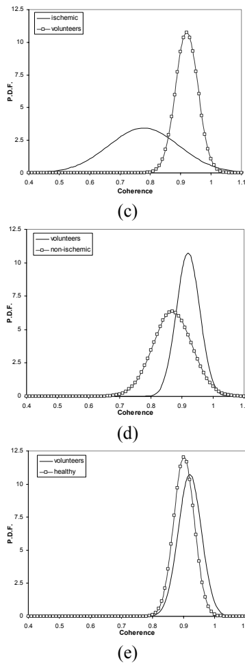
Figure 5. Normal distribution of coherence, according to the mean and SD measured. Comparison of groups in pairs.
