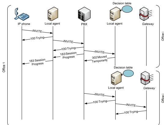
Figure 5. A call is redirected to a new office
