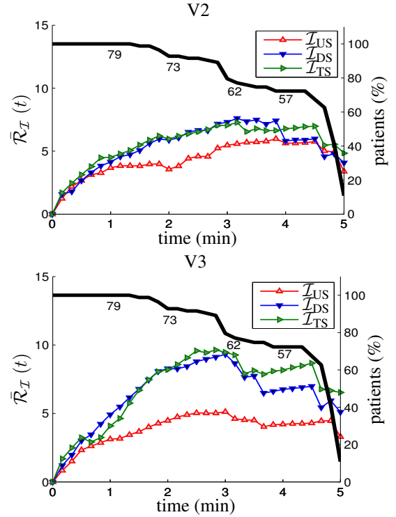
Figure 2. Averaged relative changes \mathcal{R}_{\mathcal{I}} of the three QRS slopes ( \mathcal{I}_{US} , \mathcal{I}_{DS} and \mathcal{I}_{TS} ) in leads V2 and V3. The black lines represent the percent of patients that remain under occlusion at each time instant.
