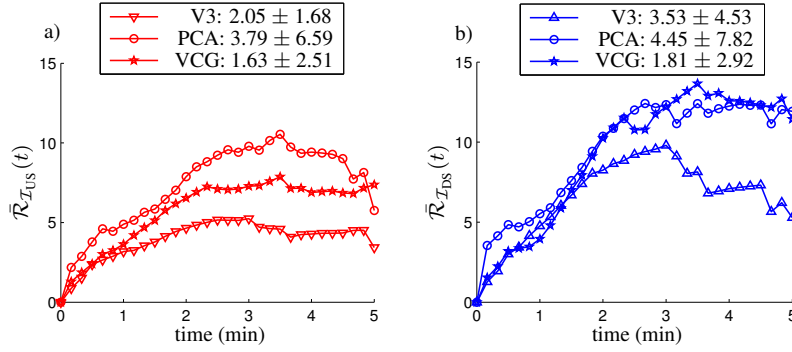
Figure 3. Evolution of the averaged relative factor of change \bar{R}_I for I_{US} (a) and I_{DS} (b) during PCI. Mean \pm SD of \sigma^I over patients in the control recordings are displayed on top of each graph.
