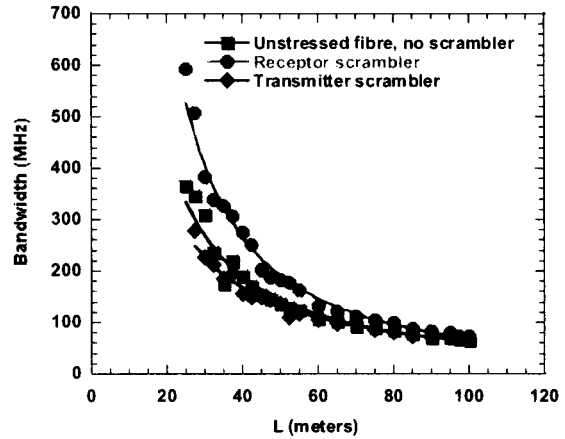
Figure 6: Bandwidth for the unstressed fibre.
