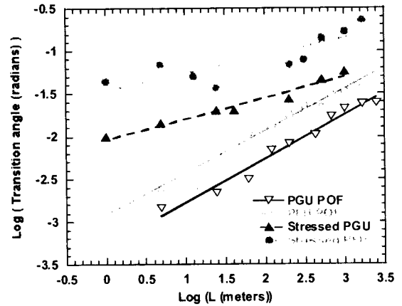
Figure 3: Mode coupling for stressed and unstressed POFs.
